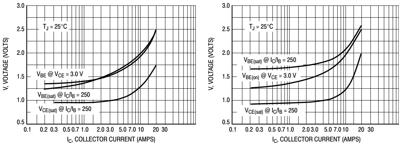
Figure 9. "On" Voltages
