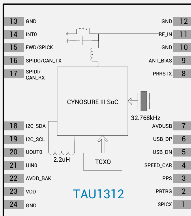
Figure 2 Block diagram
