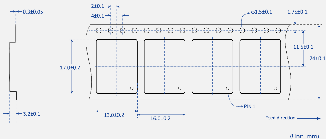
Figure 9 Tape dimensions
