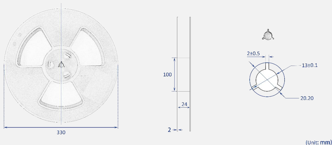
Figure 10 Reel dimensions
